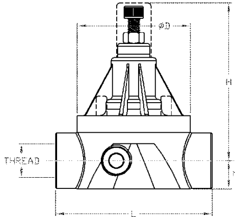
Threaded Female
