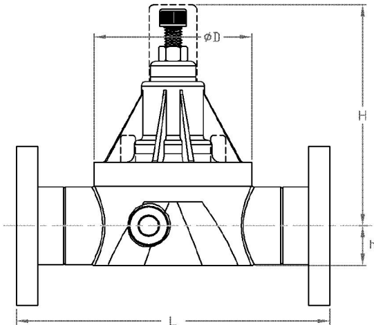
Flanged
