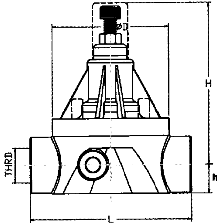
Threaded Female
