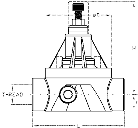
Threaded Female
