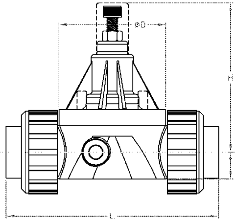
Union
